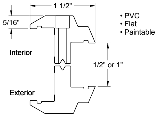
Frame Profile
