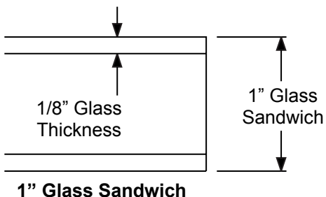
1" Glass Sandwich
