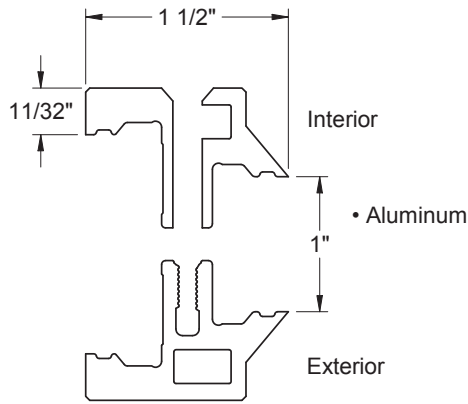
Frame Profile
