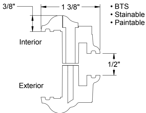
Frame Profile
