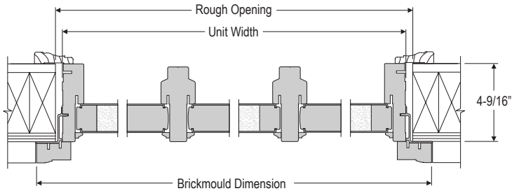
HORIZONTAL SECTION
