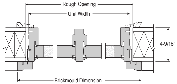
HORIZONTAL SECTION OUTSWING - FIXED/FIXED
