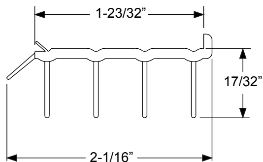
Sweep/Replacement Door Bottom
