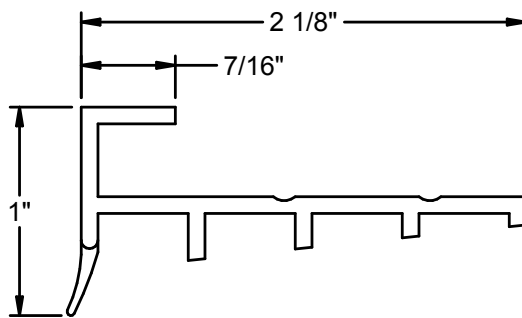
Inactive Panel Door Bottom - Composite Outswing Sill
