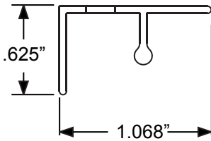
Screen Track
