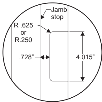
Standard Hinge
