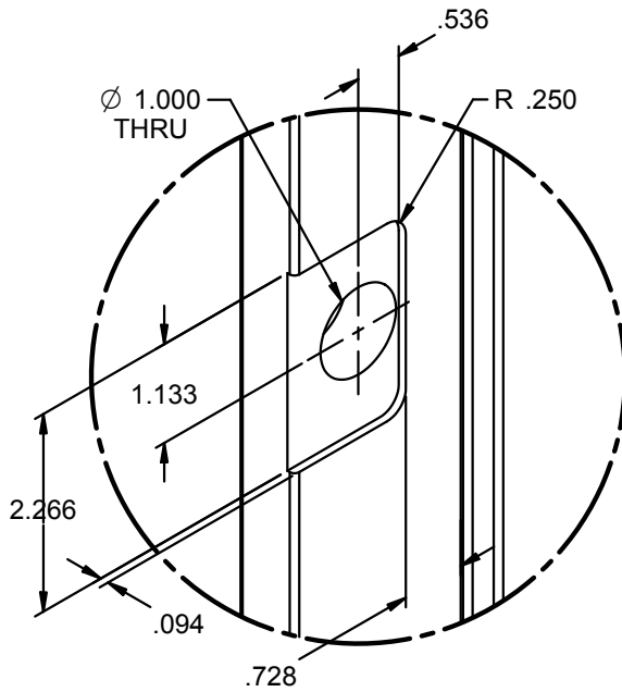
LATCH MACHINING
