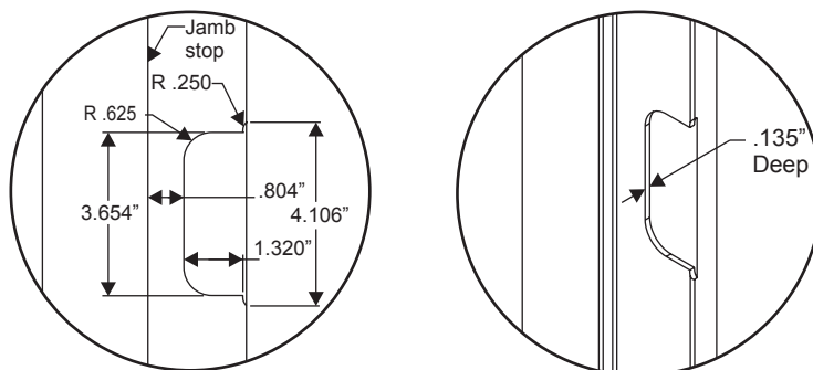
Adjustable Hinge
