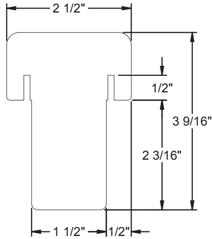
Oak, Pine, and Rot-Resistant Standard & Wide Mullion
