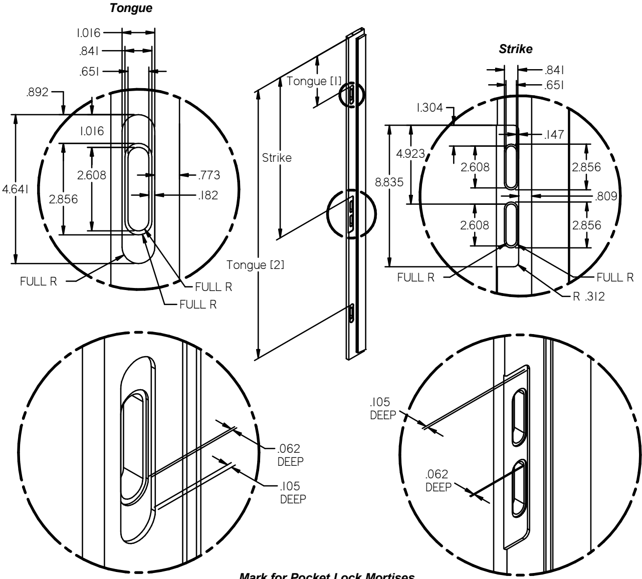
Manual Pocket - Side Jamb Lock Mortise Locations
