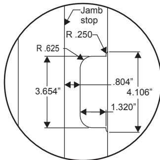
Adjustable Hinge
