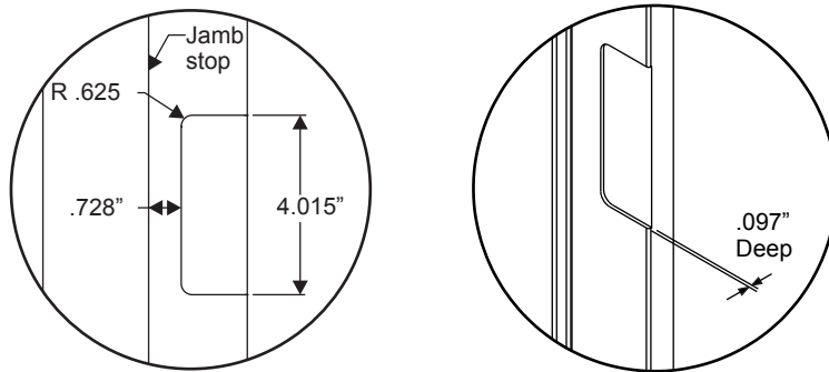
Standard Hinge
