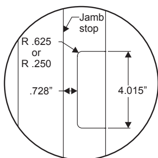
Standard Hinge
