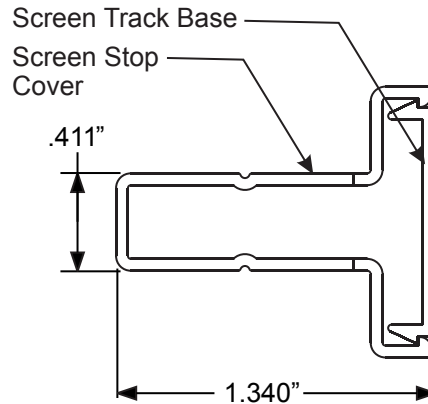
Triple Patio Screen Stop
