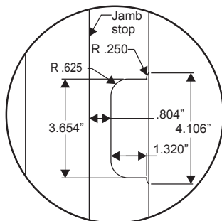
Adjustable Hinge
