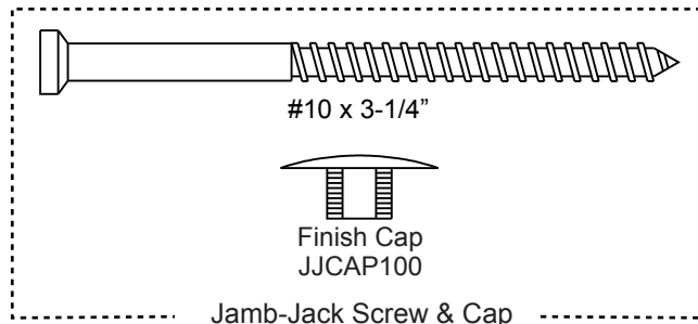
#10 x 3-1/4" Finish Cap JJCAP100 Jamb-Jack Screw & Cap JJJC06
