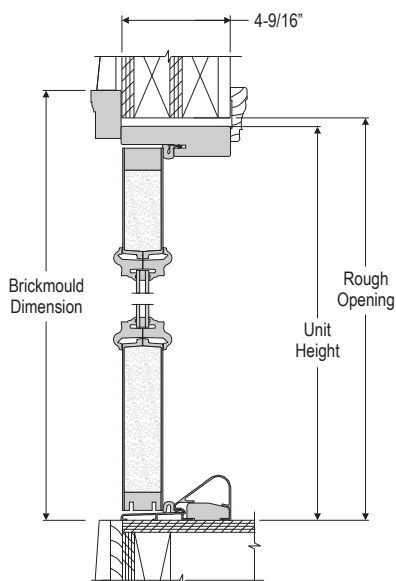
VERTICAL SECTION OUTSWING COASTAL
