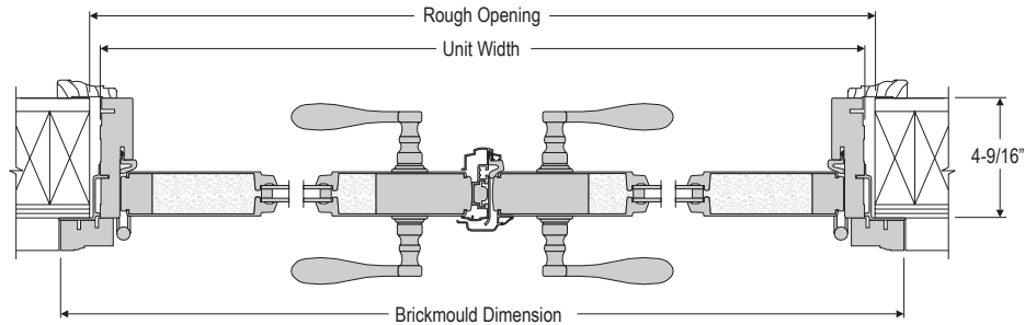
HORIZONTAL SECTION
