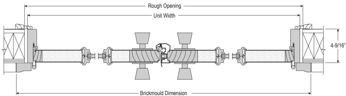
HORIZONTAL SECTION OUTSWING - DOUBLE w/ASTRAGAL (RA shown)
