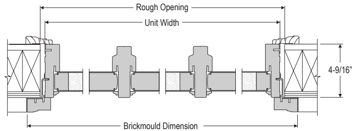
HORIZONTAL SECTION
