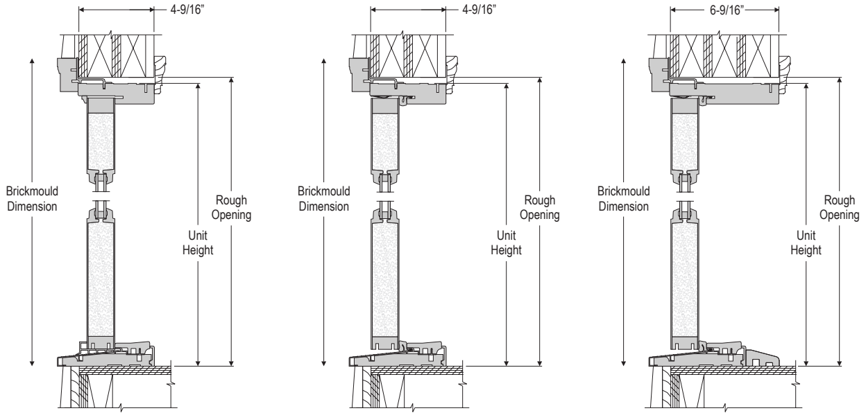
VERTICAL SECTION OUTSWING - FIXED
