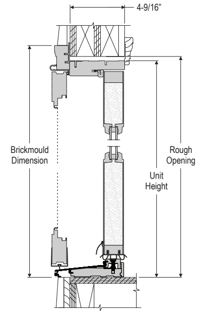
VERTICAL SECTION INSWING - DOUBLE w/ASTRAGAL w/HINGED SCREEN
