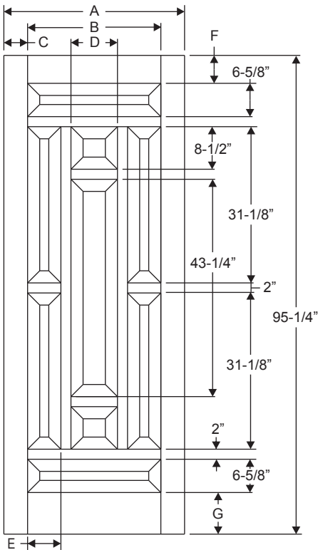
Classic-Craft Panel Dimensions
