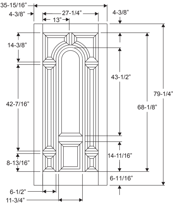
Classic-Craft Panel Dimensions
