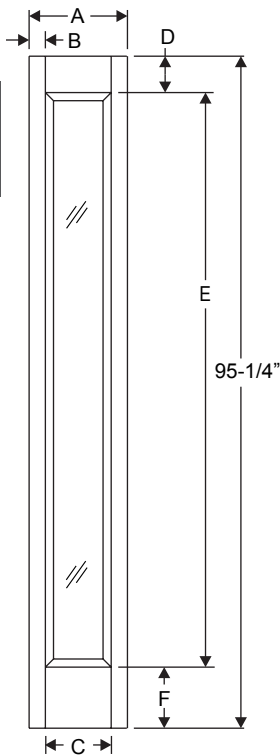
Classic-Craft Panel Dimensions
