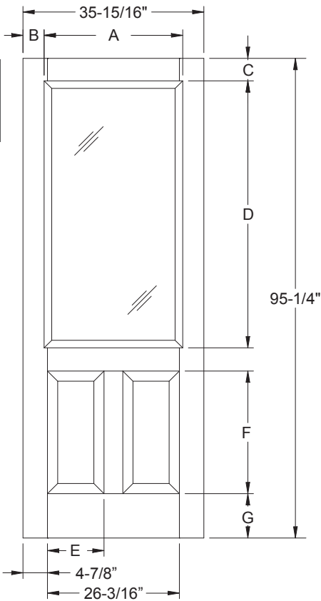
Classic-Craft Panel Dimensions
