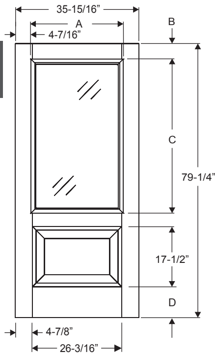
Classic-Craft Panel Dimensions
