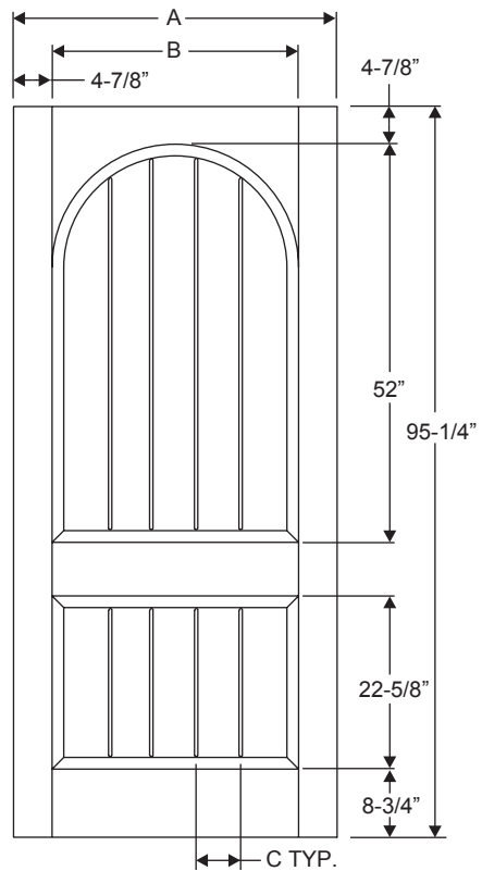
Classic-Craft Panel Dimensions
