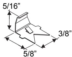
Retaining Clip
