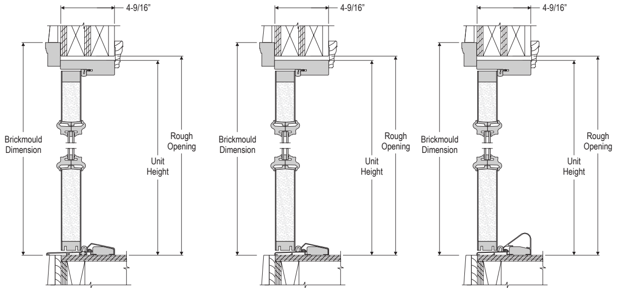
VERTICAL SECTION OUTSWING THERMAL BREAK
