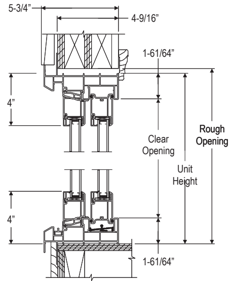
VERTICAL SECTION - ALL OTHERS
