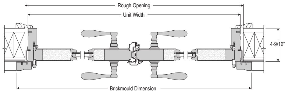
HORIZONTAL SECTION
