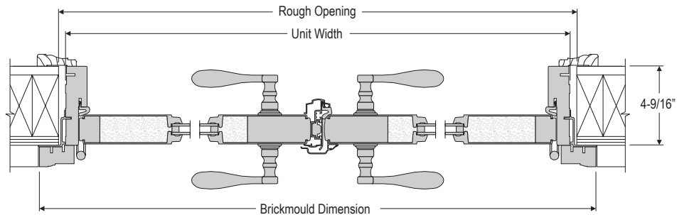
HORIZONTAL SECTION
