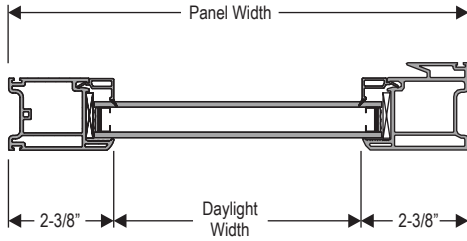
HORIZONTAL PANEL SECTION Scale: 3" = 1'
