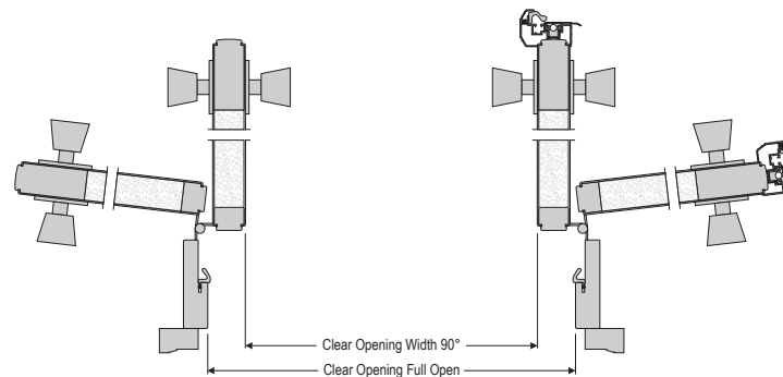
HORIZONTAL SECTION (French) (Hinged off jamb or mullion)
