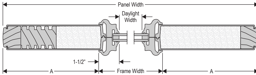
FIBER CLASSIC AND SMOOTH-STAR HORIZONTAL PANEL SECTION
