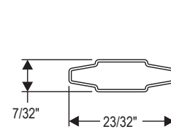
CONTOUR GBG GRILLE SECTION
