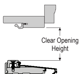
VERTICAL SECTION INSWING G
