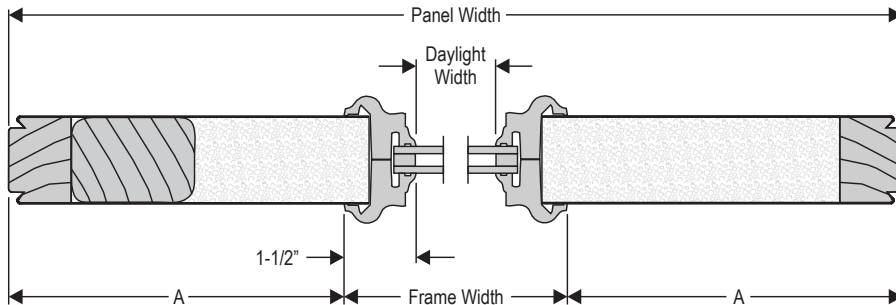
STEEL HORIZONTAL PANEL SECTION
