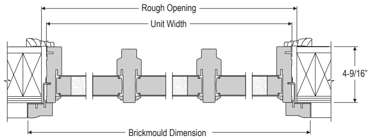
HORIZONTAL SECTION
