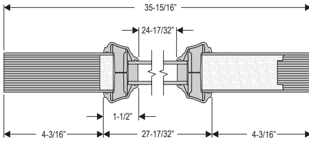
HORIZONTAL PANEL SECTION
