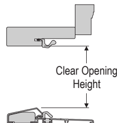
VERTICAL SECTION OUTSWING G
