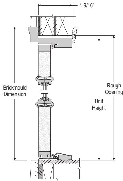
VERTICAL SECTION OUTSWING NO THERMAL BREAK
