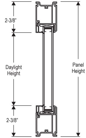
VERTICAL PANEL SECTION Scale: 3" = 1'
