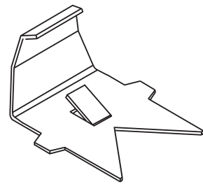
Part # RPFGGC Flushed-Glazed Wood Grille Metal Clip
